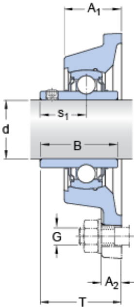
FY 1.3/16 TF/VA228 Bearing 2D drawings and 3D CAD models
