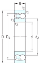
Cylindrical bore
