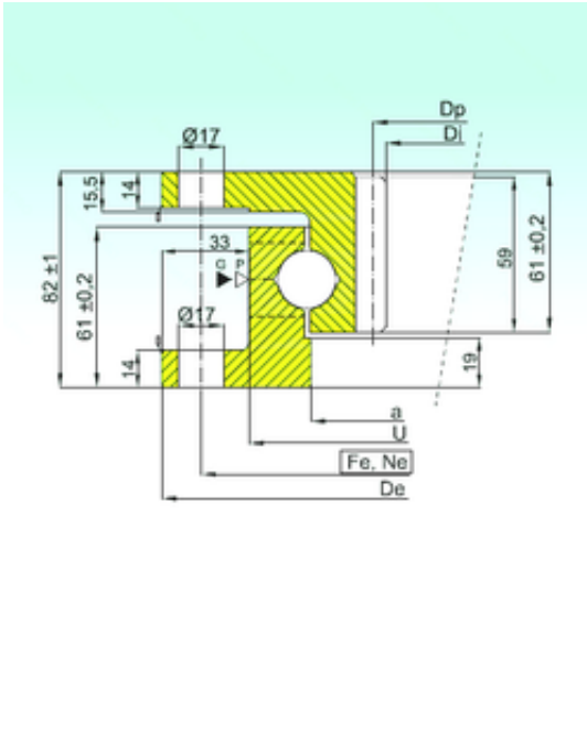
ZK.22.0800.100-1SN Bearing 2D drawings and 3D CAD models
