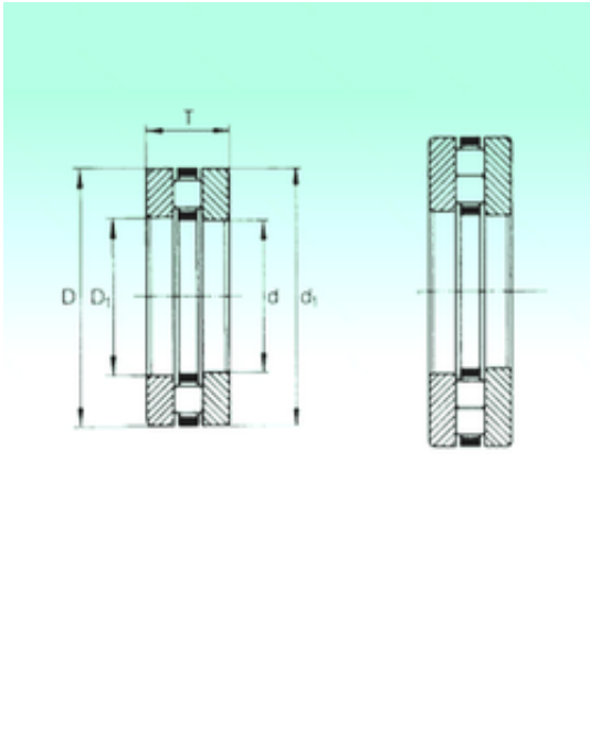
89412TN Bearing 2D drawings and 3D CAD models
